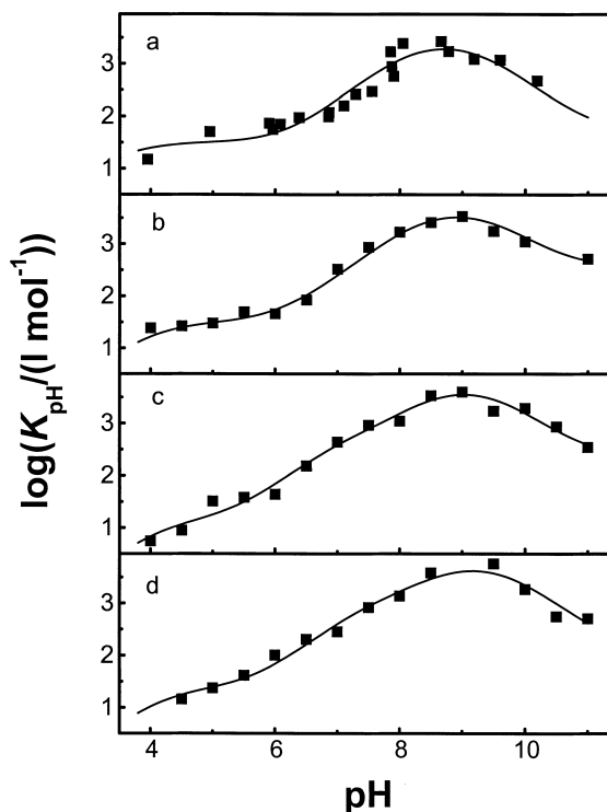
Fig. 3. Plot of \log K_{\text{pH}} vs pH for the PLP-TRP system in a) water, b) 24 wt% ethanol, c) 44 wt% ethanol and d) 62 wt% ethanol. Curves calculated using Eq. 7 and data from Table 1.
