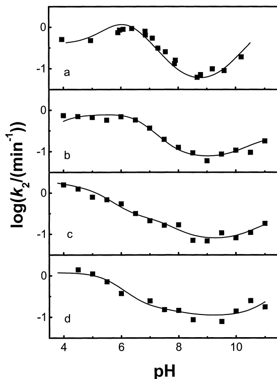
Fig. 2. Plot of \log k_2 vs pH for the PLP-TRP system in a) water, b) 24 wt% ethanol, c) 44 wt% ethanol and d) 62 wt% ethanol. Curves calculated using Eq. 6 and data from Table 1.
