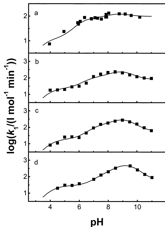
Fig. 1. Plot of \log k_1 vs pH for the PLP-TRP system in a) water, b) 24 wt% ethanol, c) 44 wt% ethanol and d) 62 wt% ethanol. Curves calculated using Eq. 5 and data from Table 1.
