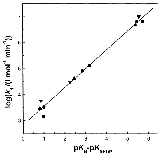
Fig. 4. Plot of \log k_i^1 as a function of (pK_N - pK_{(i+1)P}) for the corresponding species in water (■) and in aqueous media with different ethanol contents: 24 wt% (●), 44 wt% (▲) and 62 wt% (▼)
